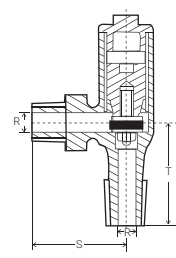
FERRULE WITH MALE THREADED * (BRASS INSERT)
