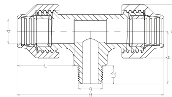
COMPRESSION TEE WITH BRANCH MALE THREADED
