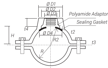
METAL SERVICE SADDLE
