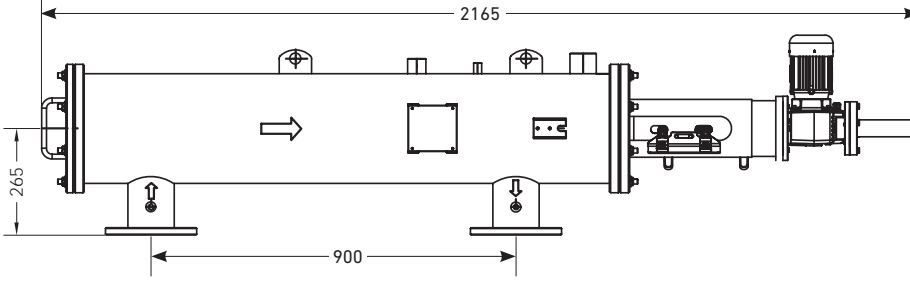
4" HEO FILTER ASSEMBLY
