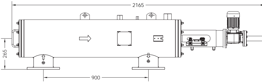
6" HEO FILTER ASSEMBLY
