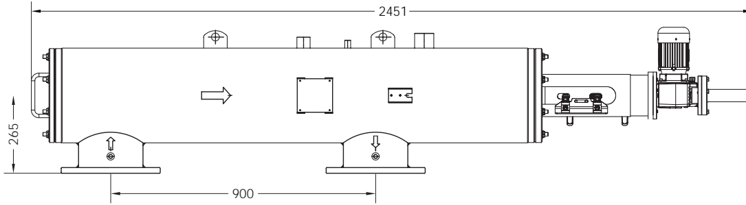
8" HEO FILTER ASSEMBLY
